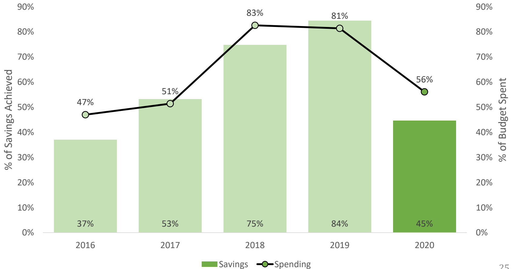
Energy Star HVAC - Annual Gas Savings and Spending Performance to Goal Through Q3 (2016-2020)
